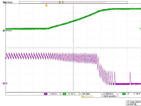
V_{IN} = 48\text{ V} V_{OUT} = 12\text{ V} Load = 0 A to Short Figure 9-8. Short-Circuit Recovery
