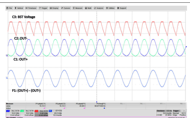
Figure 7-3. Full Scale Output 30 V PP at 100 Hz
