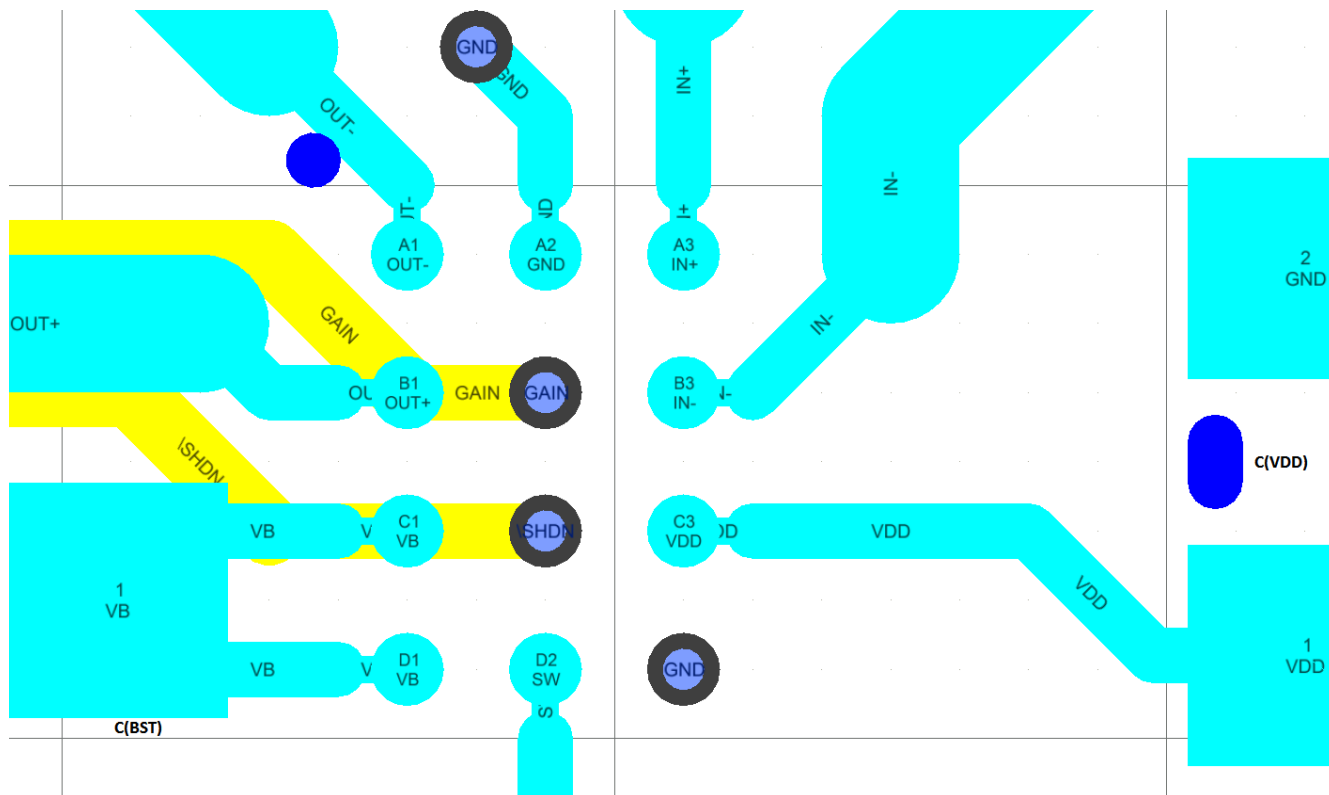
Figure 7-4. Example Layout
