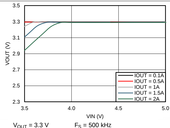
Figure 50. Drop-Out Curve
