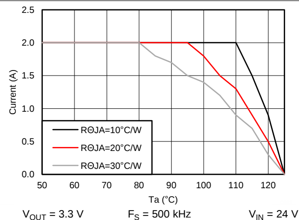
Figure 52. Derating Curve
