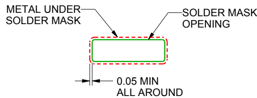
SOLDER MASK DETAILS PADS 1-16
