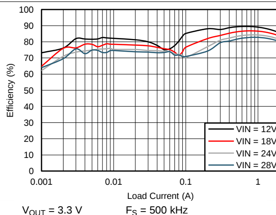
Figure 48. Efficiency
