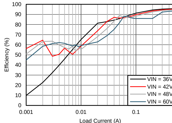
Figure 78. Efficiency
