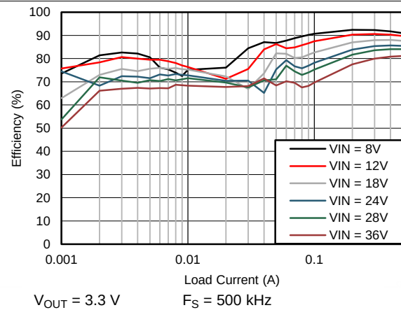
Figure 48. Efficiency
