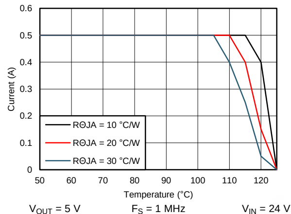
Figure 70. Derating Curve
