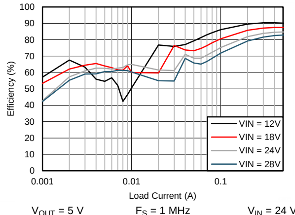
Figure 66. Efficiency
