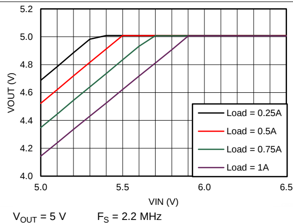
Figure 17. Dropout Curve
