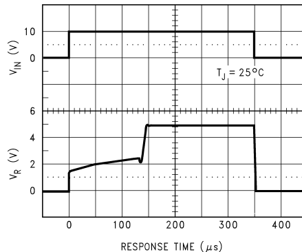
Figure 5-7. Input Voltage Step Response LM4050-N-5
