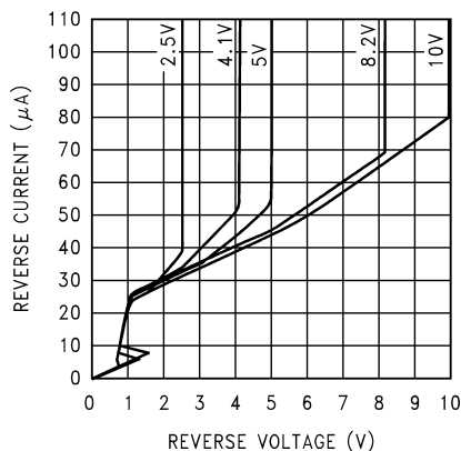
Figure 5-3. Reverse Characteristics and Minimum Operating Current
