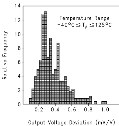
Figure 5-5. Thermal Hysteresis
