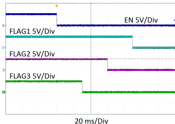
Figure 8-3. Powerdown Sequence for LM3880MF-1AB
