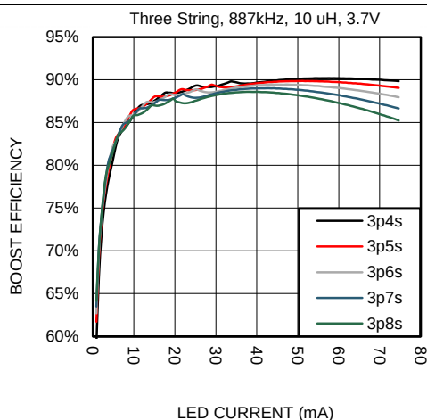
Figure 46. Boost Efficiency vs Series LEDs
