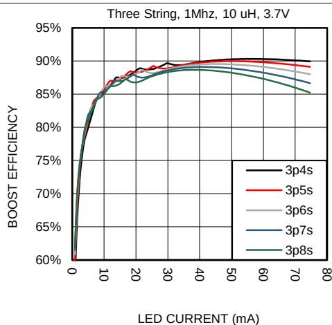
Figure 44. Boost Efficiency vs Series LEDs
