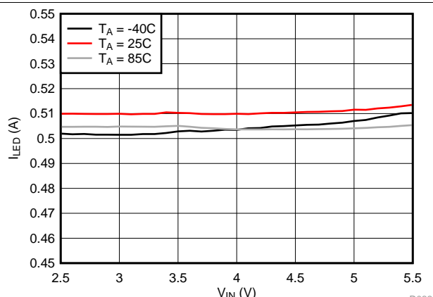
Figure 9. LED Current vs Input Voltage
