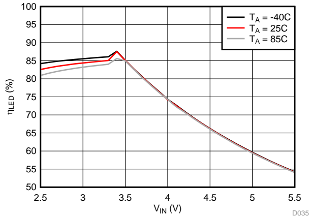
LM3648TT f_{SW} = 4 \text{ MHz} Torch Brightness Code = 0x59 V_{LED} = 3.03 \text{ V} D035
