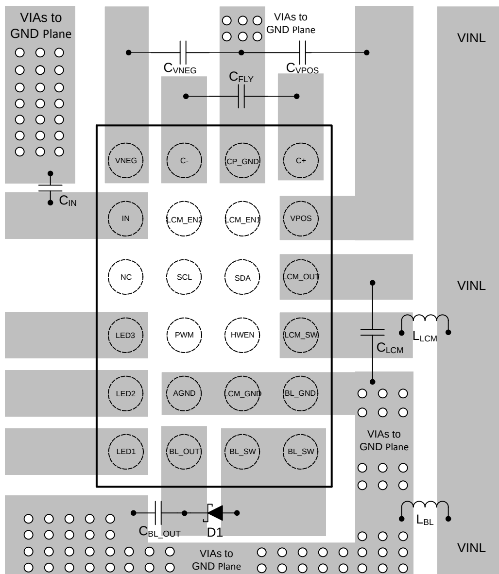
Figure 175. LM36273 Layout Example
