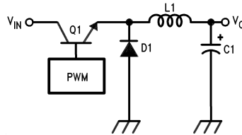
Figure 27. Basic Buck Regulator
