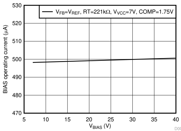
Figure 7-9. I OPERATING(BIAS) Including RT Current vs V BIAS
