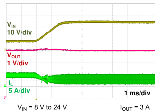
Figure 6-18. Line Transient
