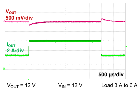
Figure 6-16. Load Step (Buck-Boost)
