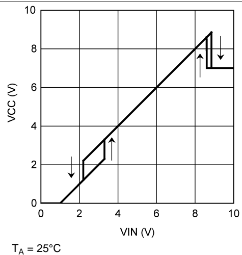
Figure 12. V_{CC} vs V_{IN}
