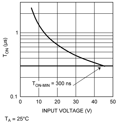
Figure 7. T_{ON} vs V_{IN} , R_{ON} = 100 \text{ k}\Omega
