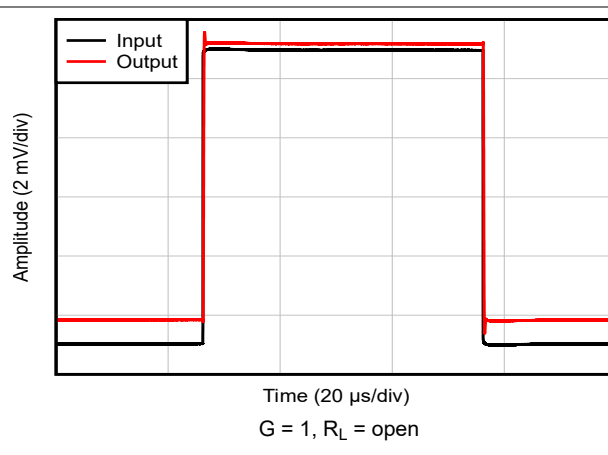
Figure 5-26. Small-Signal Step Response, G = 1
