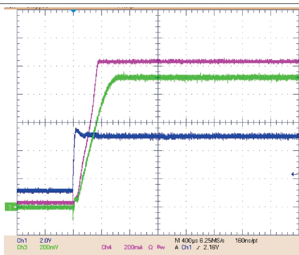
Figure 22. V_{IN} = 5.0\text{ V} , V_{OUT} = 0.9\text{ V} , I_{load} = 1\text{ A} at -40°C
