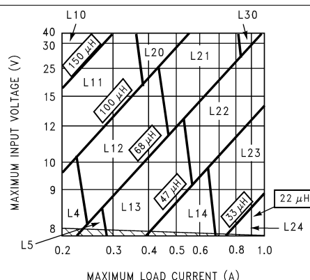
Figure 24. LM2672, 5-V Output
