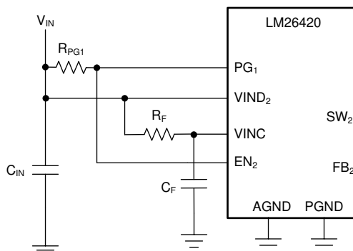
Figure 7-4. PG 1 Controlling V OUT2
