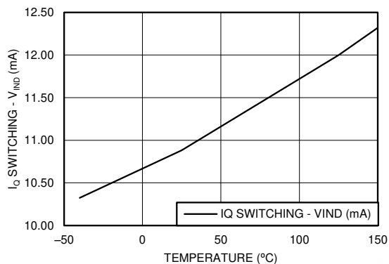
Figure 5-19. I_Q (Quiescent Current) vs Temperature (Q0 Grade)
