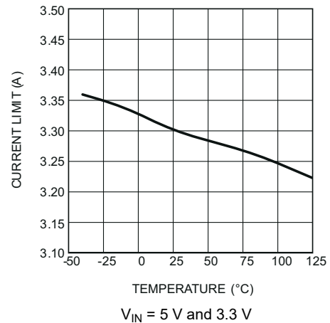
Figure 5-16. Current Limit vs Temperature V_{IN} = 5\text{ V and } 3.3\text{ V}
