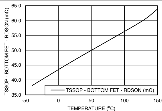
Figure 5-24. R_{DS(on)} Bottom vs Temperature (Q0 Grade)
