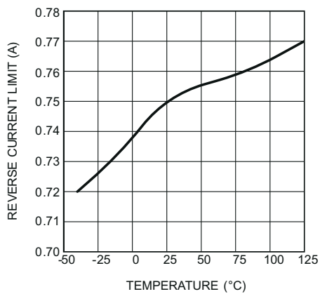
Figure 5-17. Reverse Current Limit vs Temperature
