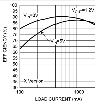
Figure 5-4. Efficiency vs Load
