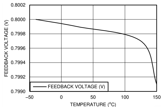
Figure 5-20. V_{FB} vs Temperature (Q0 Grade)
