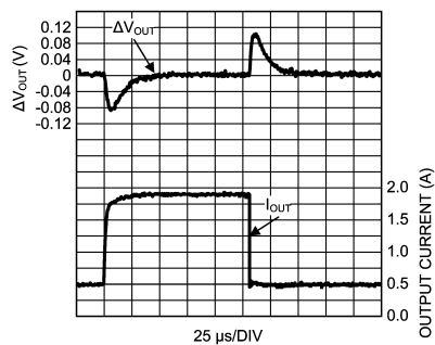
Figure 7-10. Load Transient Response
