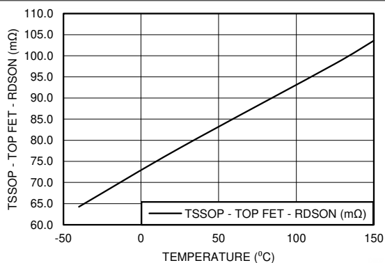
Figure 5-23. R_{DS(on)} Top vs Temperature (Q0 Grade)
