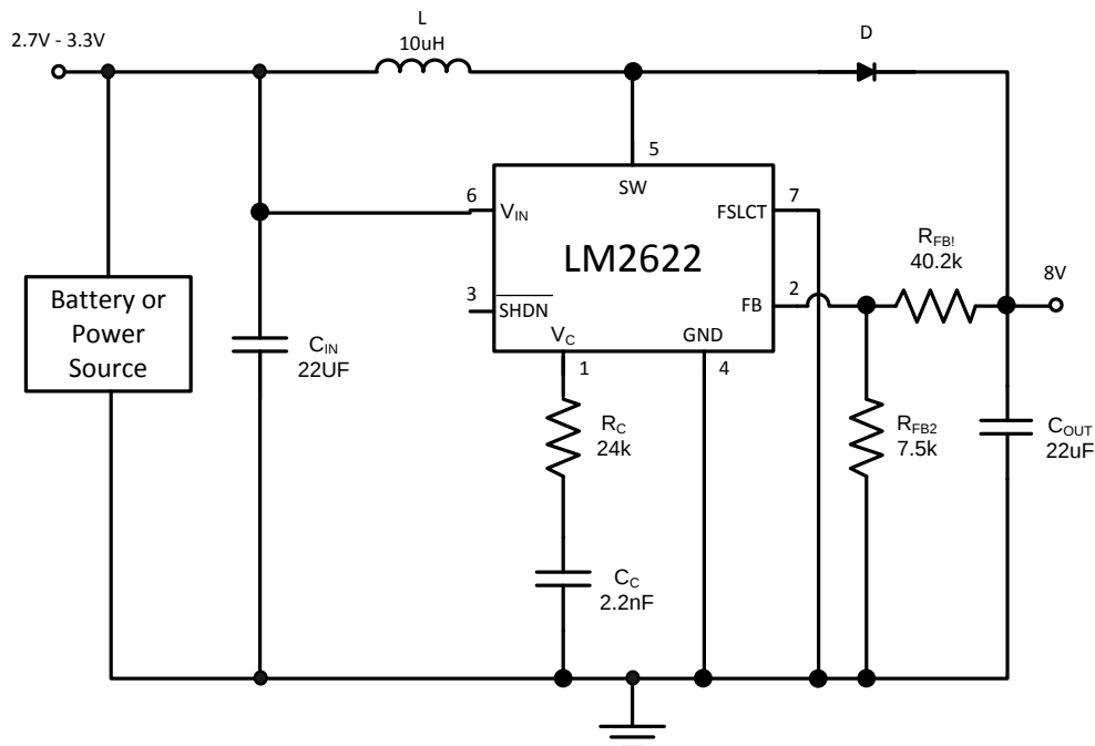
Figure 1. 600 kHz Operation
