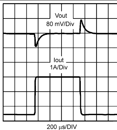
Figure 21. Load Transient Response
