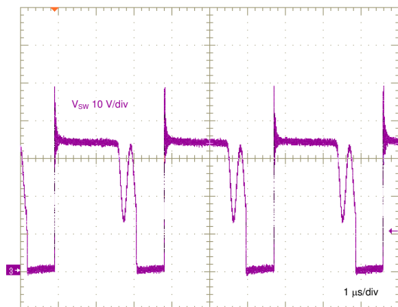
Figure 8-23. Switch Voltage, Medium Load
