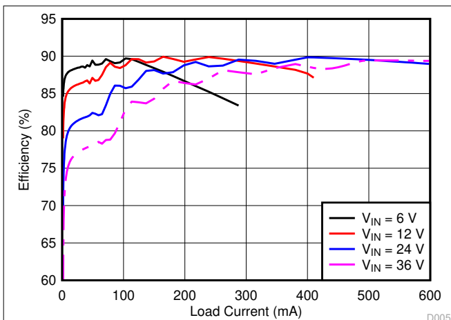
Figure 8-17. Efficiency (Linear Scale)
