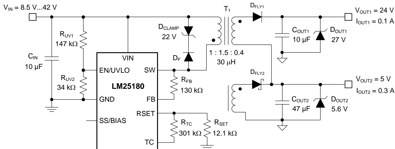
Figure 45. Schematic for Design 3 With V_{IN(nom)} = 24\text{ V} , V_{OUT1} = 24\text{ V} , V_{OUT2} = 5\text{ V}
