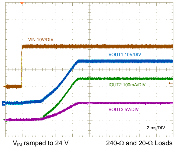
Figure 47. Start-Up Characteristic
