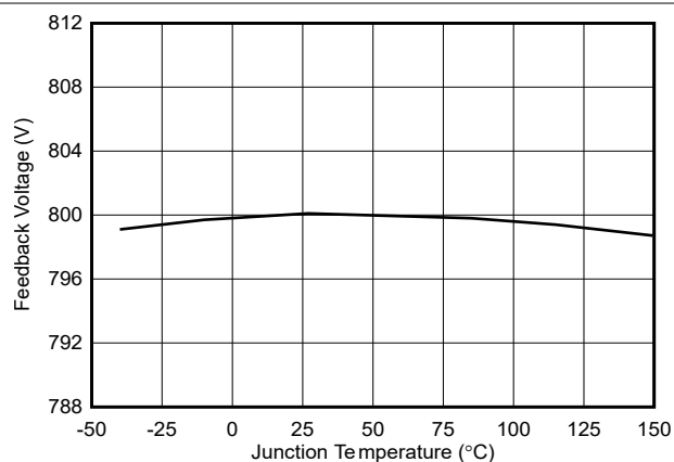
Figure 7-8. Feedback Voltage vs Temperature
