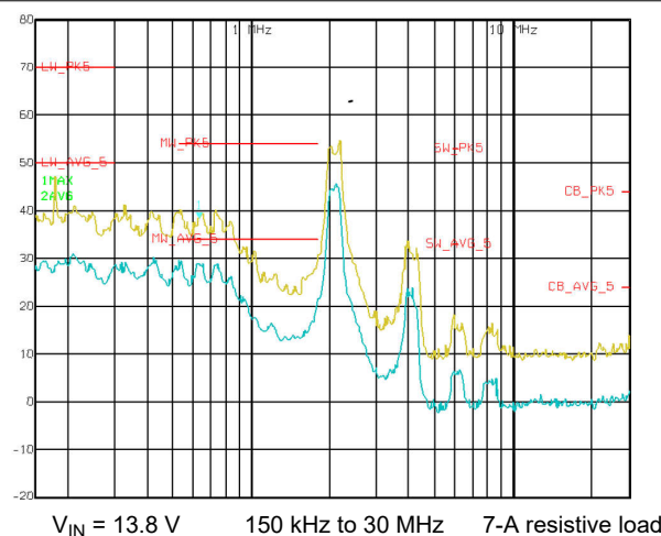
Figure 9-16. CISPR 25 Class 5 Conducted EMI
