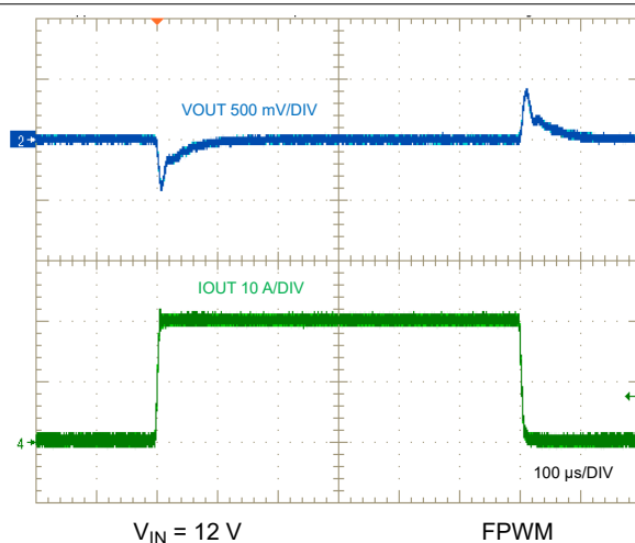
Figure 9-34. Load Transient, 0 A to 20 A
