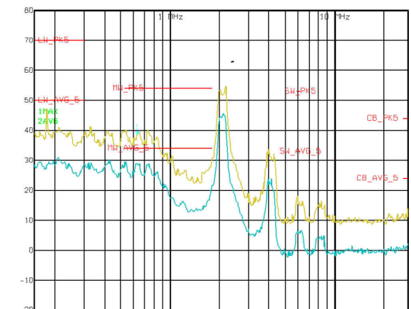
CISPR 25 EMI Performance, 150 kHz to 30 MHz
