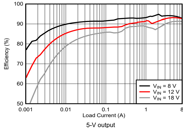
Figure 9-6. Efficiency vs I_{OUT} , Log Scale
