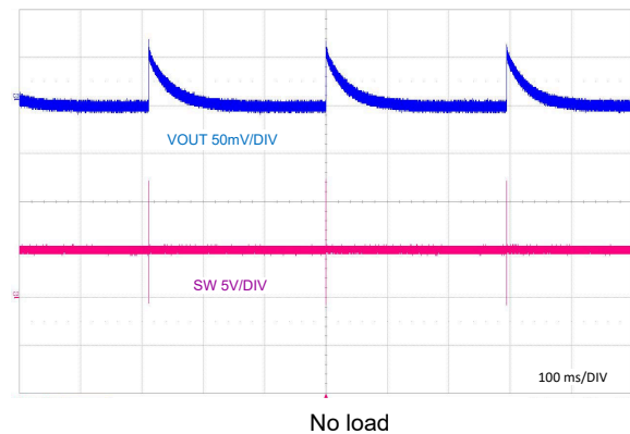
Figure 9-21. PFM Switching
