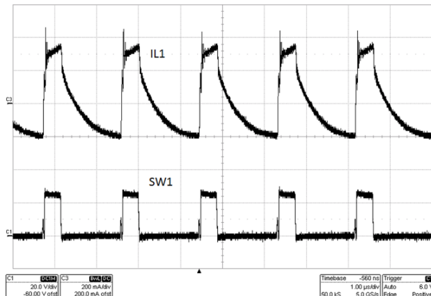
Figure 8-9. Steady State Waveform ( V_{IN} = 24\text{ V} , I_{OUT1} = 100\text{ mA} , I_{OUT2} = 200\text{ mA} )
