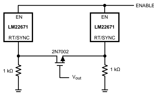
Figure 14. Self-Synchronizing Setup
