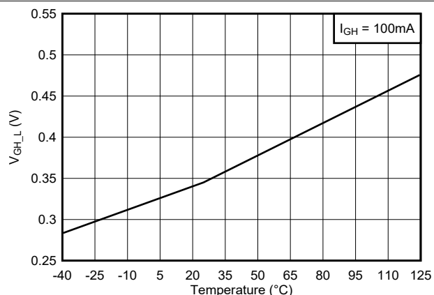
Figure 6-10. GH Output Low Voltage vs Temperature
