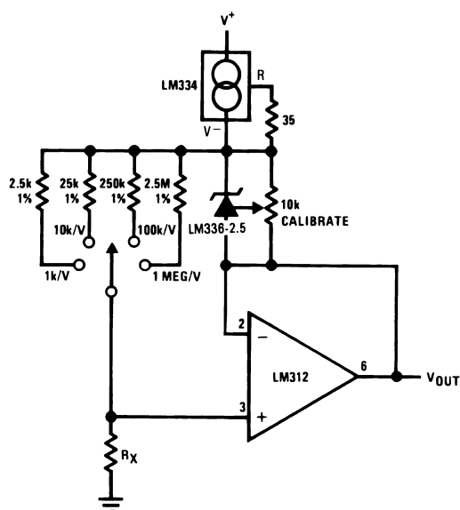
Figure 19. Linear Ohmmeter
