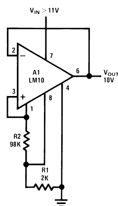
Figure 42. Best Regulation
