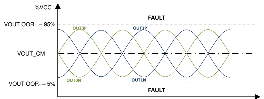
Figure 6-4. Out of Operation Fault Detection Range at the Output
