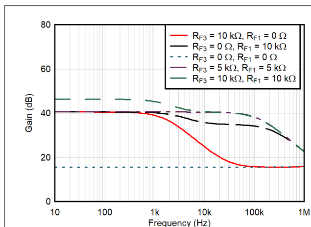
Figure 9-8. Gain/Phase
