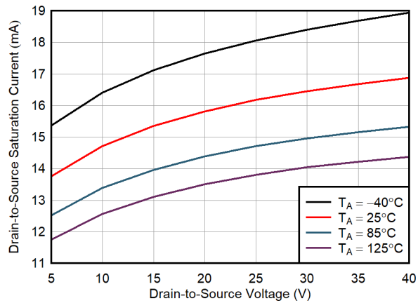
Figure 6-9. I_{DS} vs Drain-to-Source Voltage
