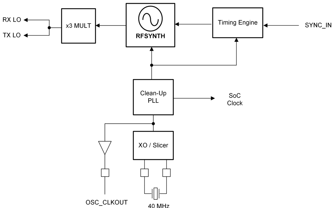
Figure 8-2. Clock Subsystem
