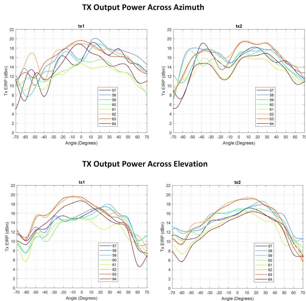
Figure 7-9. Transmitter Antenna Radiation Pattern
