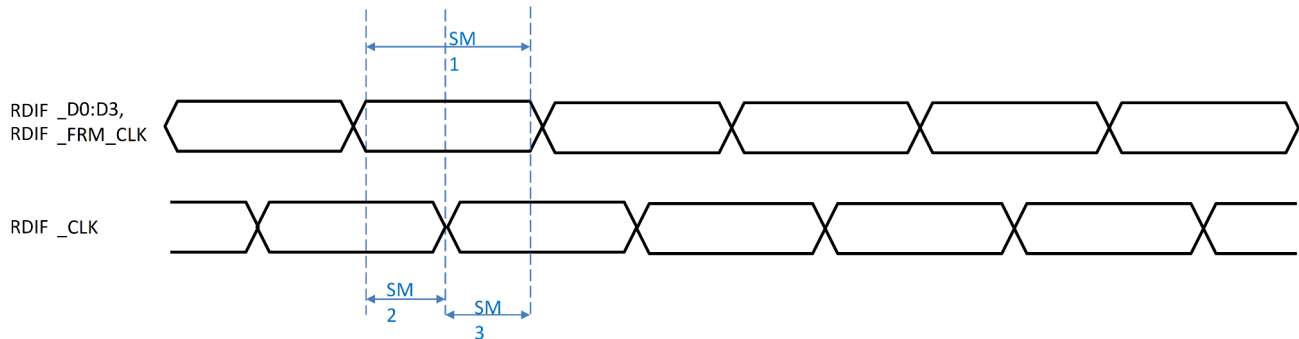
Figure 7-18. RDIF Timing Requirements
