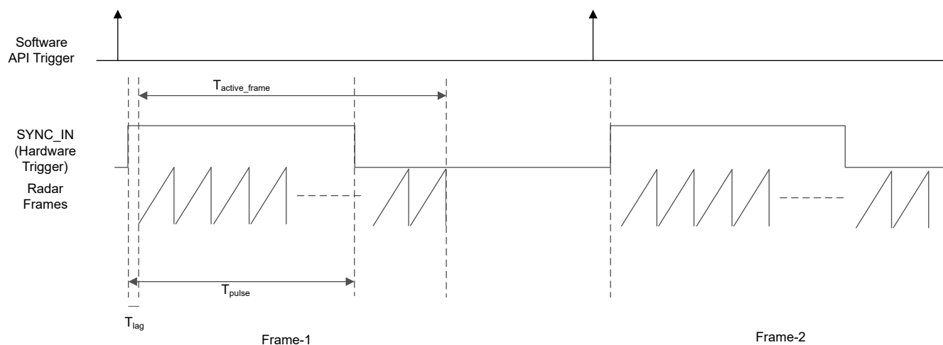
Figure 7-12. Sync In Hardware Trigger
