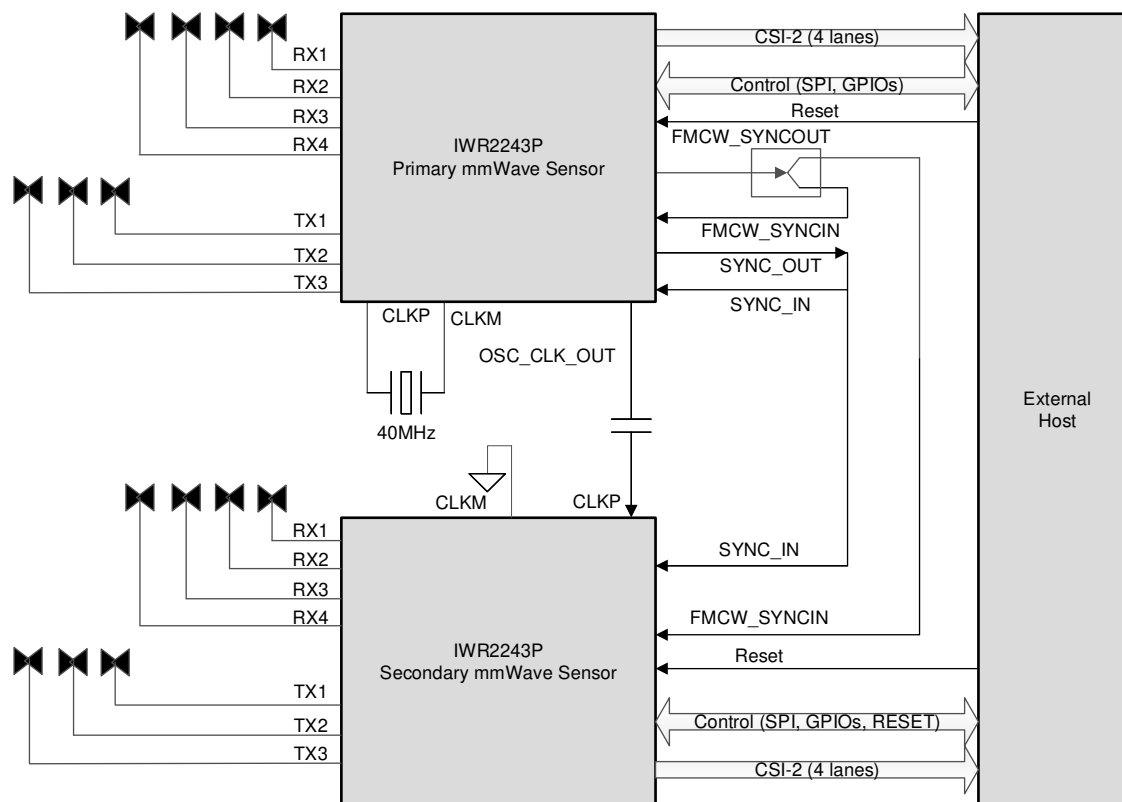
Figure 11-1. Imaging Radar using Cascade Configuration
