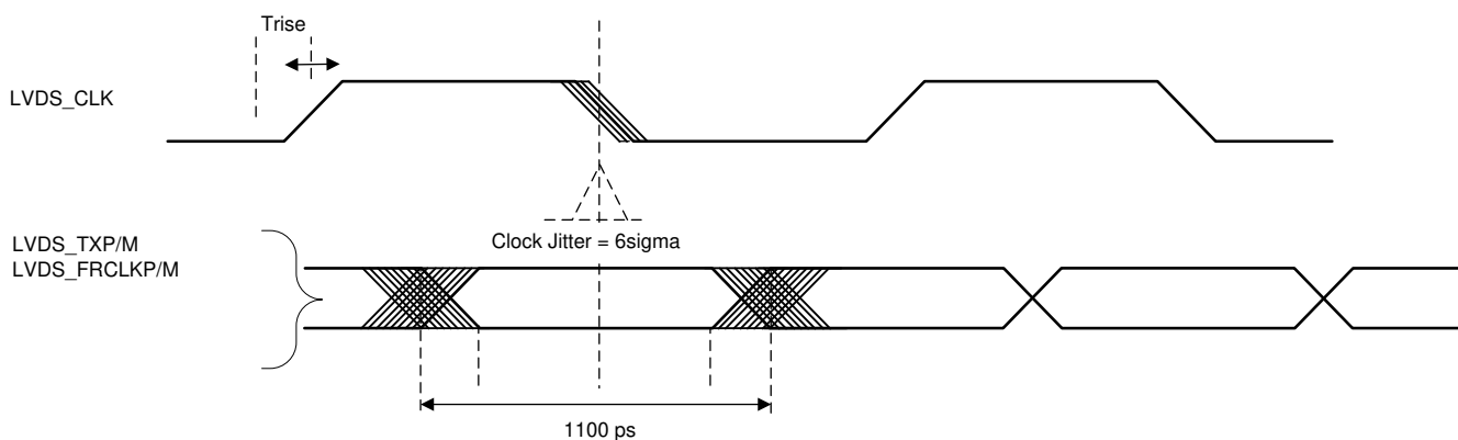
Figure 8-11. Timing Parameters
