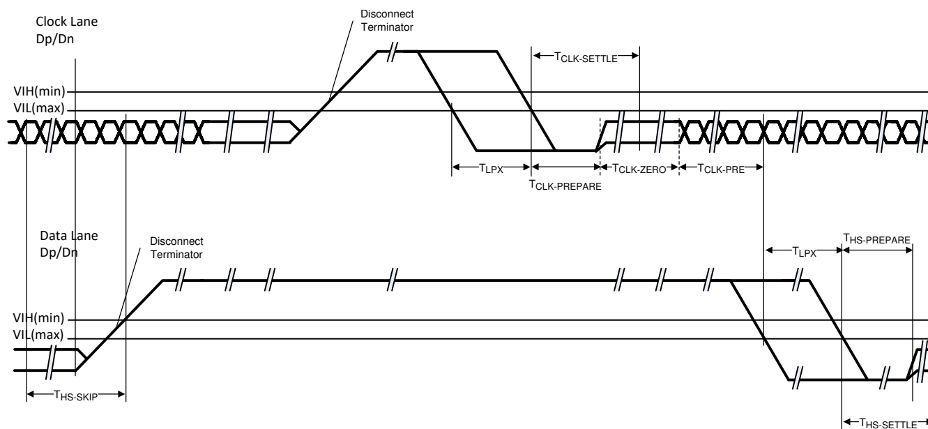
Figure 8-13. High-Speed Data Transmission Burst
