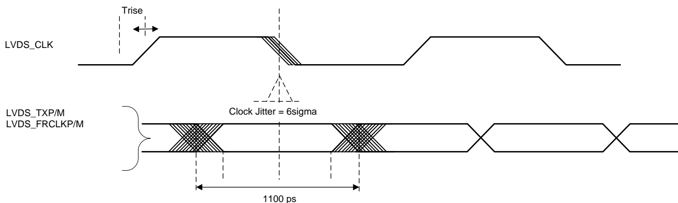
Figure 5-13. Timing Parameters
