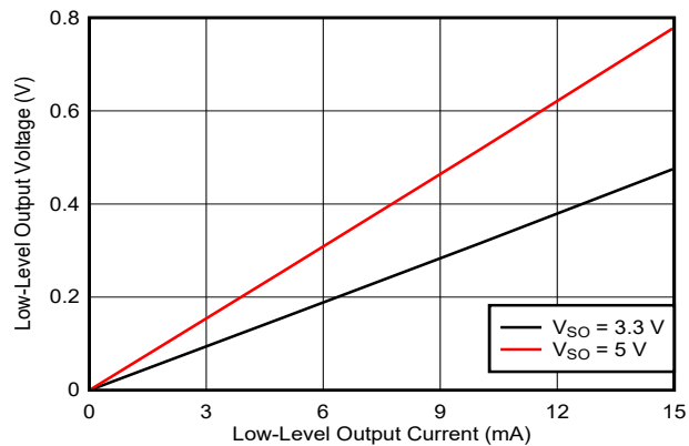
Figure 7-16. Low-Level Output Voltage vs Low-Level Output Current
