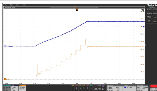
Figure 7-18. Soft Start at 10-mA Load For V_{ISOOUT} = 3.3 V
