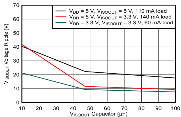
Figure 7-28. V_{ISOOUT} Ripple Voltage vs Load Capacitor
