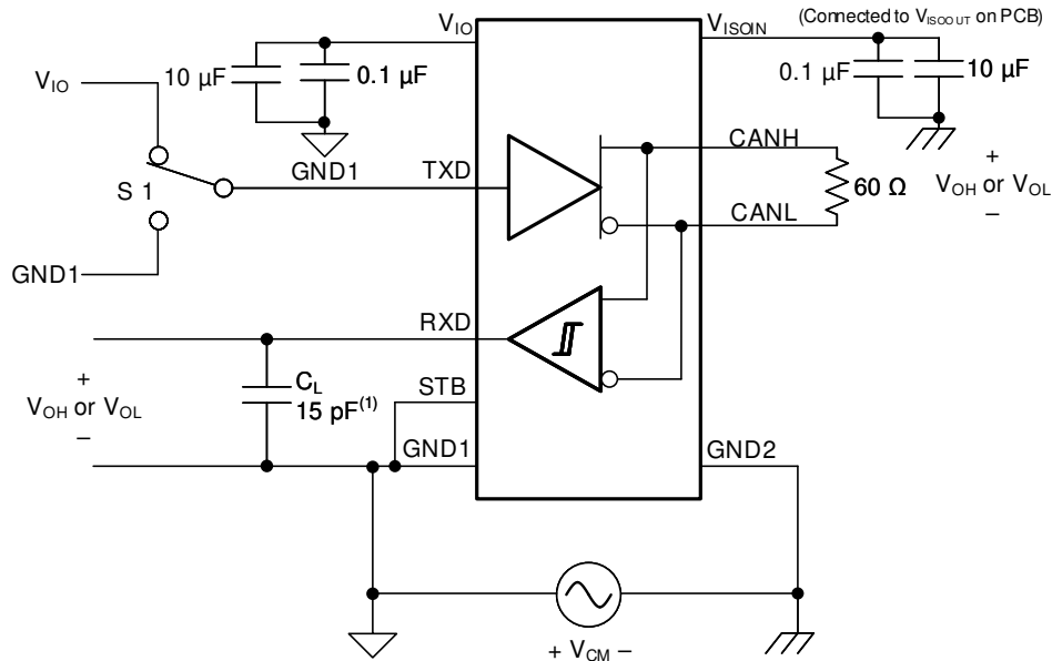
Figure 9-9. Common-Mode Transient Immunity Test Circuit
