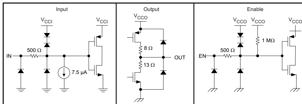
Figure 15. Device I/O Schematics
