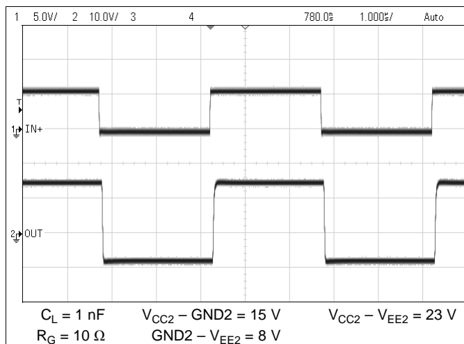
Figure 52. Normal Operation - Bipolar Supply
