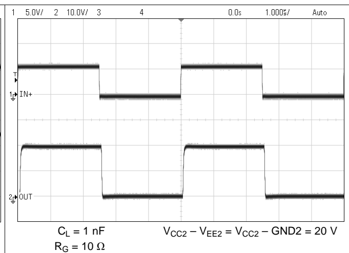
Figure 53. Normal Operation - Unipolar Supply
