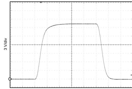
Figure 7-10. Output Transient Waveform
