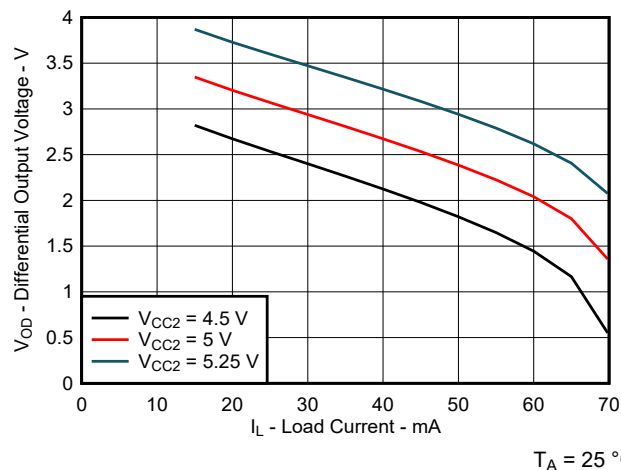
Figure 6-12. Driver Differential Output Voltage vs Load Current
