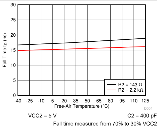
Figure 6-7. Side 2: Output Fall Time vs Free-Air Temperature
