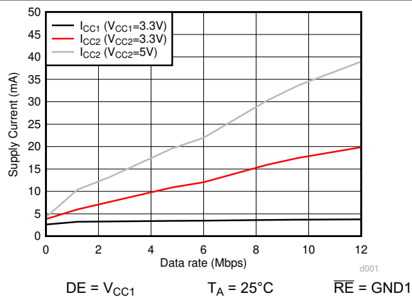
Figure 7-6. ISO143x Supply Current Vs. Data Rate - No Load
