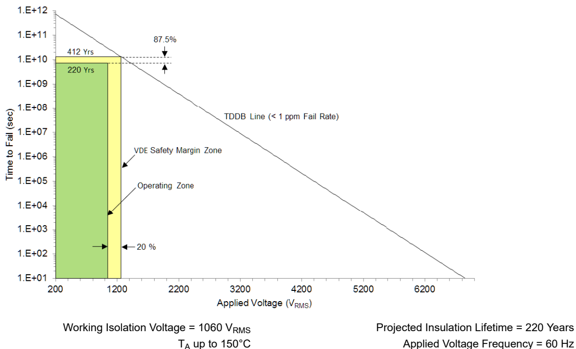
Figure 10-7. Insulation Lifetime Projection Data
