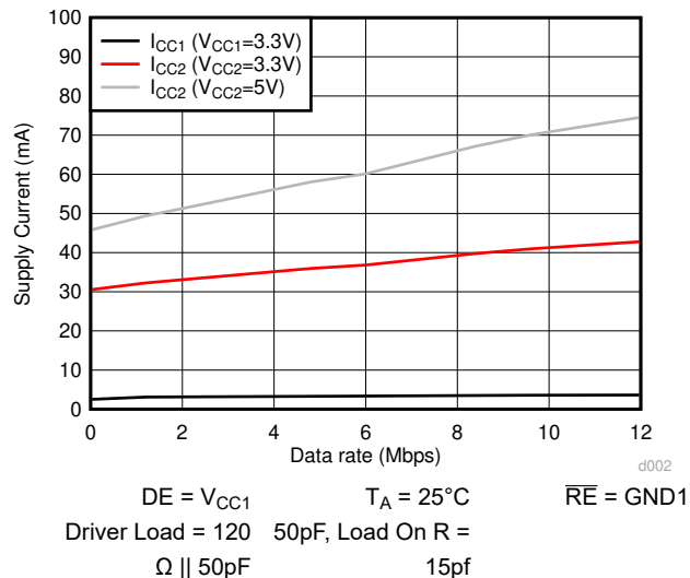
Figure 7-7. ISO143x Supply Current Vs. Data Rate - 120 \Omega ||50pF Load
