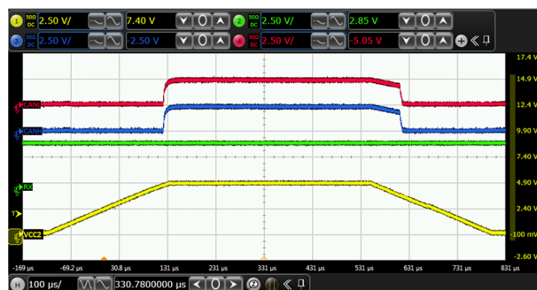
Figure 6-14. Glitch Free Power Up on V_{CC2} – CAN Bus Remains Recessive
