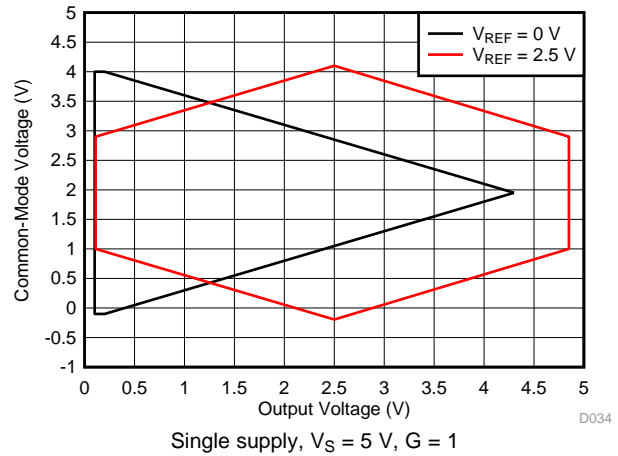
Figure 14. Input Common-Mode Voltage vs Output Voltage
