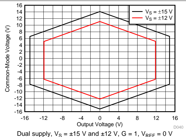
Figure 18. Input Common-Mode Voltage vs Output Voltage
