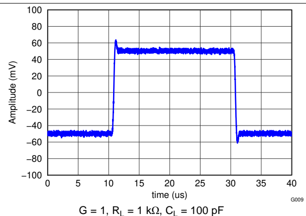
Figure 52. Small-Signal Response
