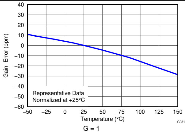
Figure 33. Gain Error vs Temperature
