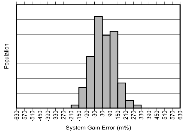
Figure 5-12. INA791B-Q1 Gain Error Production Distribution
