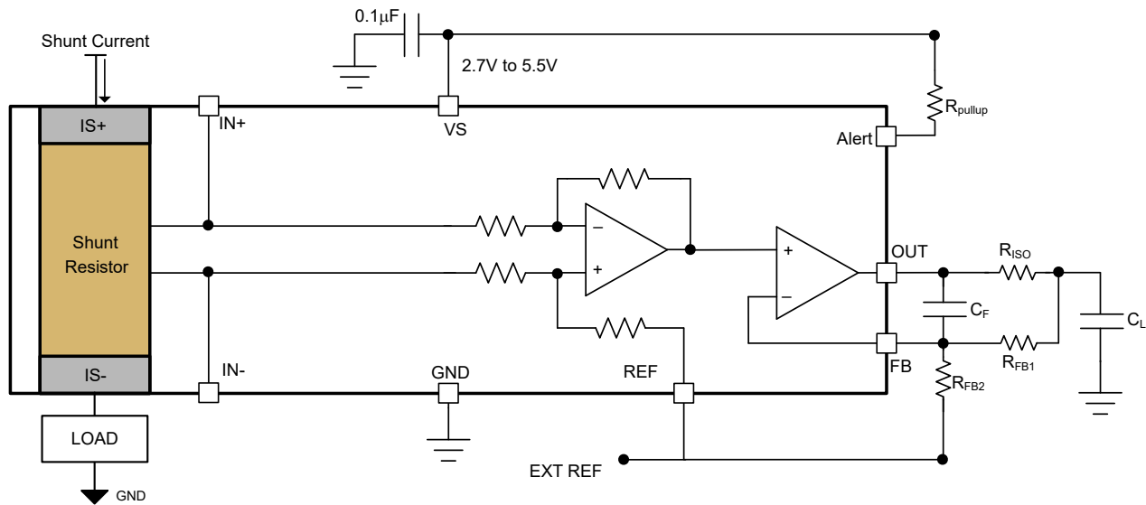
Figure 7-5. INA791x-Q1 With RISO-Dual-Feedback
