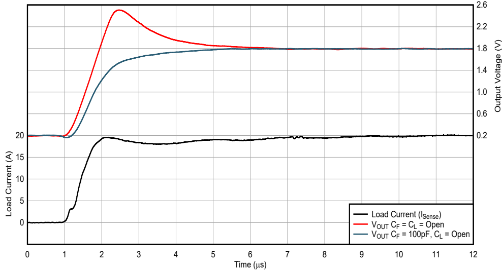
Figure 7-6. INA791x-Q1 Load Step Responses Before and After RISO Dual Feedback for Adjustable Gain of 1
