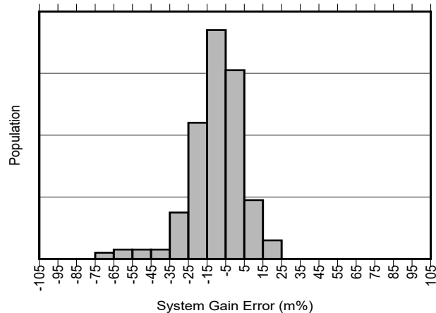
Figure 5-11. INA791A-Q1 Gain Error Production Distribution
