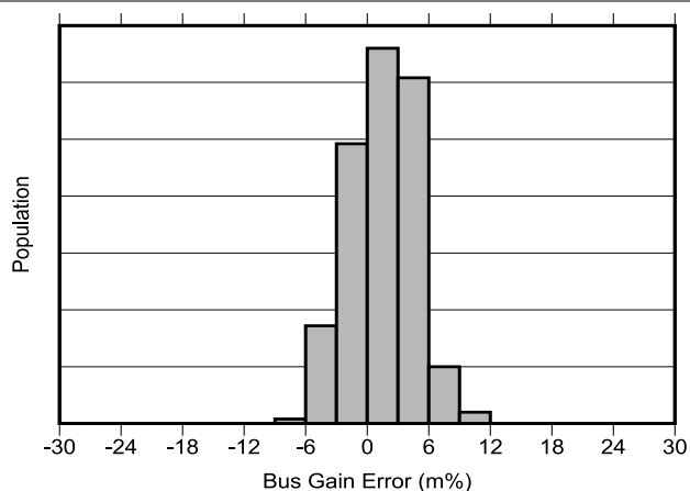
Figure 5-11. Bus Input Gain Error Production Distribution
